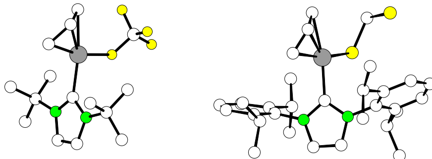
Molecular structures of (\eta^3\text{-C}_3\text{H}_5)\text{Pd}(\text{C}\{\text{N}(\text{t-Bu})\text{CH}\}_2)(\text{BF}_4) ( 9 ) and [(\eta^3\text{-C}_3\text{H}_5)\text{Pd}(\text{C}\{\text{N}(\text{C}_6\text{H}_3\text{-2,6-}^i\text{Pr}_2)\text{CH}\}_2)(\text{CH}_2\text{Cl}_2)]\text{PF}_6 ( 10 ) (cation only)
