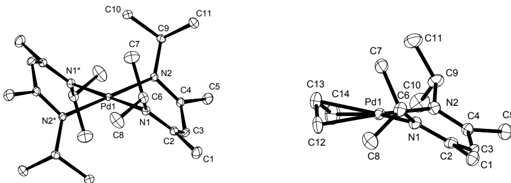
Molecular structures of \text{Pd}(^i\text{Pr}_2\text{-nacnac})_2 ( 12b ) and (\eta^3\text{-C}_3\text{H}_5)\text{Pd}(^i\text{Pr}_2\text{-nacnac}) ( 12c )
